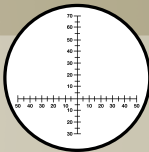
Mil Ranging Reticle
