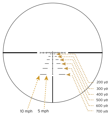
PLEX S7 RETICLE
