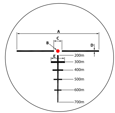
RAPID DOT 5.56, 7.62 RETICLE SUBTENSION
