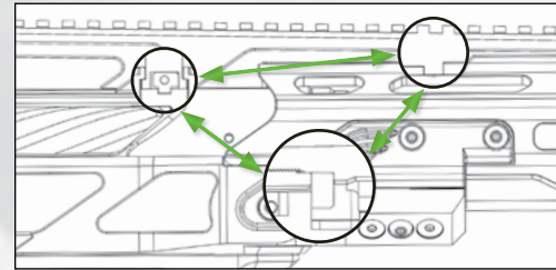
Triple recoil lug system
