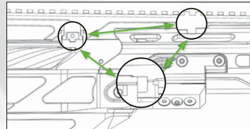
Triple recoil lug system
