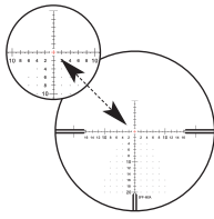
Illuminated reticle ZMOAi-T20 (thin line) For Conquest V4
